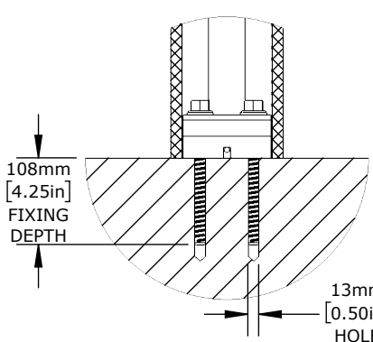
FlexCore 4 Fixing Detail
