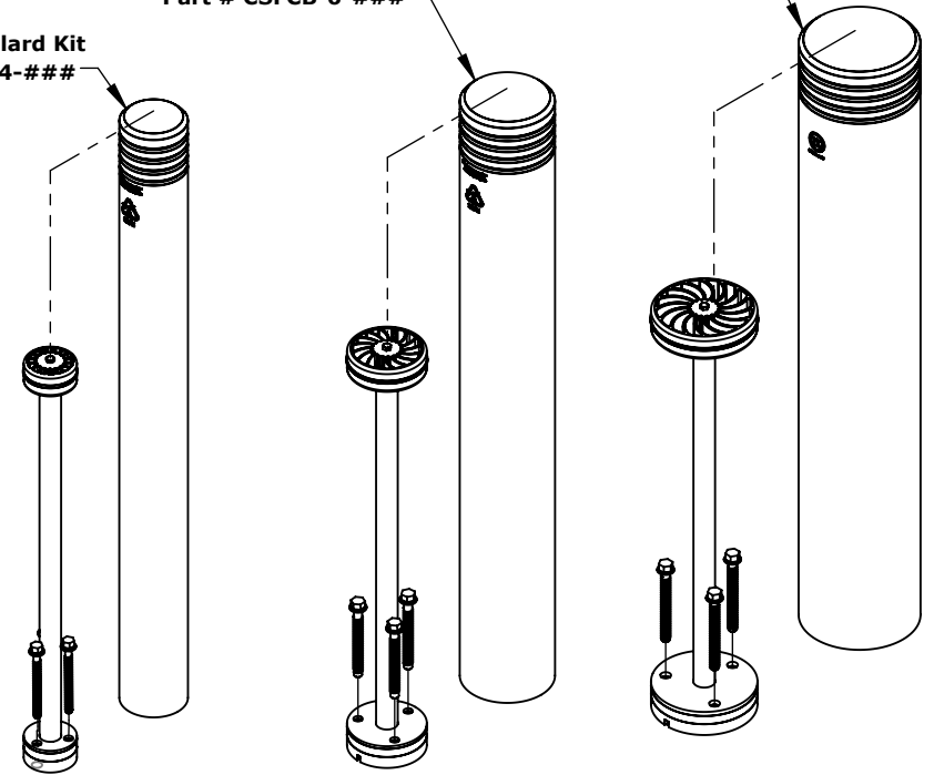
FlexCore 6 Bollard Kit Part # CSFCB-6-###
