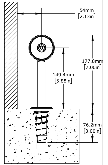
Mounting Details SCALE: 1:8
