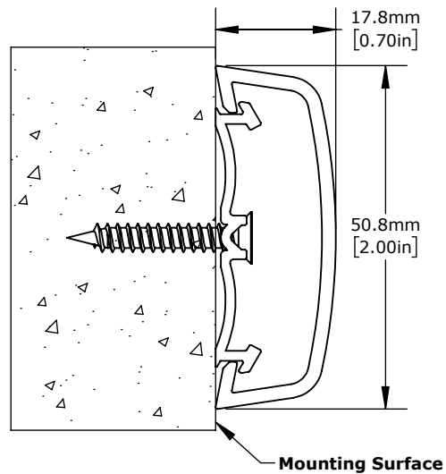
Profile View As-Installed SCALE: 1:1
