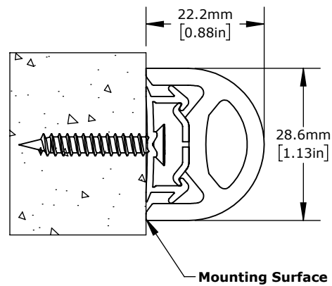
Profile View As-Installed SCALE:1:1
