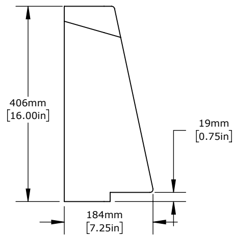
16" Shock Absorbing Rack Guard for Wide Racks
