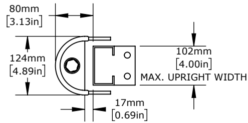
Top View - Standard Racks
