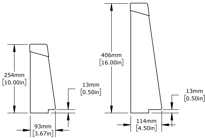
10" Shock Absorbing Rack Guard for Standard Racks
