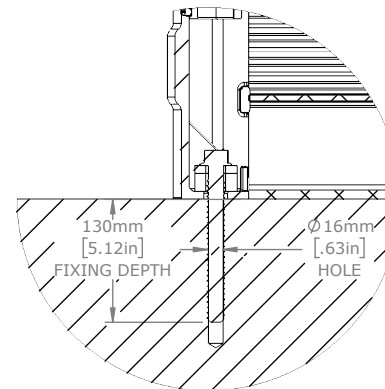
Fixing Detail
