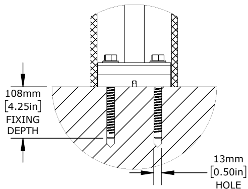
FlexCore 6 Fixing Detail
