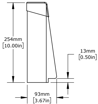
10" Shock Absorbing Rack Guard
