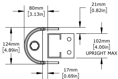
Top View - Both Sizes
