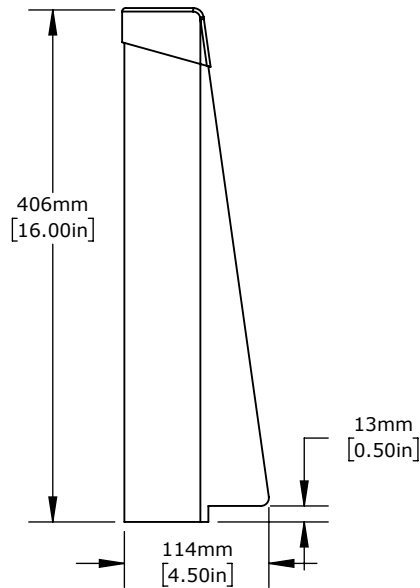
16" Shock Absorbing Rack Guard
